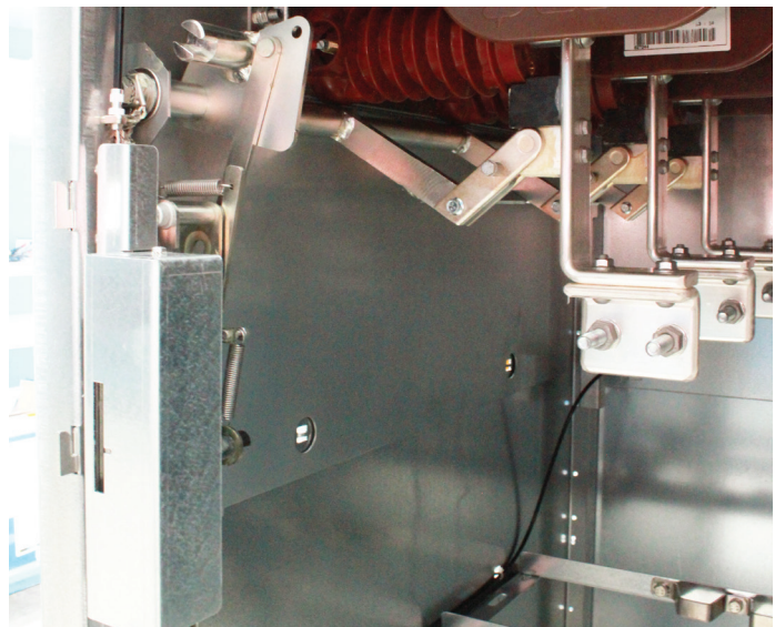
Arc-Killer
